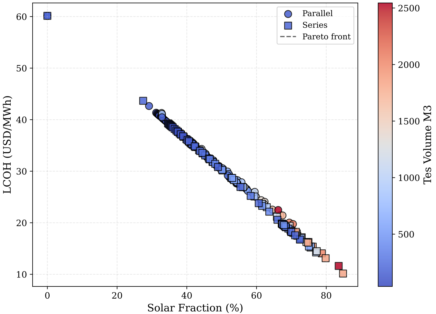
LCOH vs Solar Fraction — Pareto Frontier
