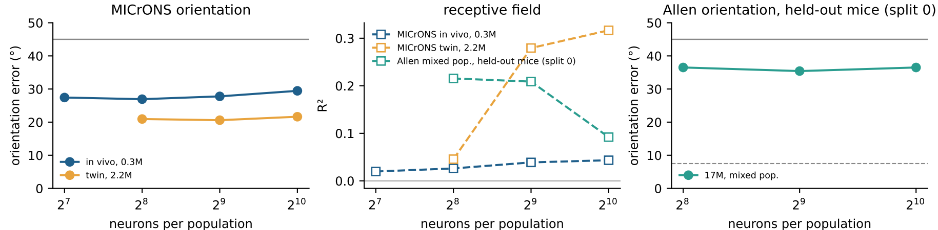
Fig. A2 Population size saturates by 512 neurons (MICrONS) and 256 (Allen)
