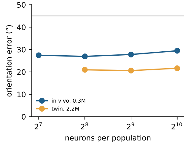
MICrONS orientation
