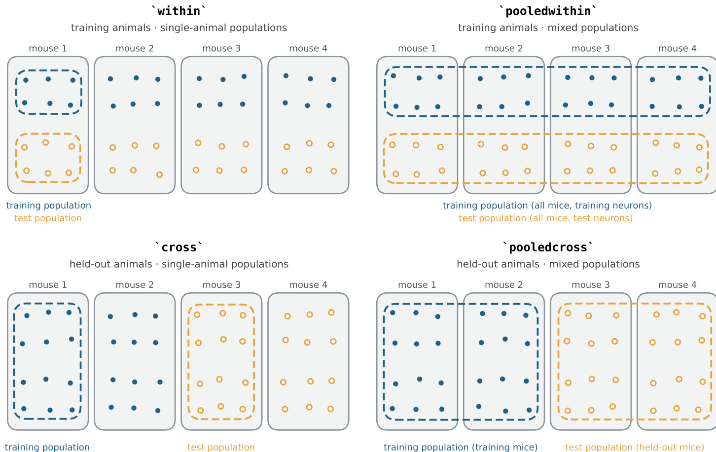
Fig. 4 Allen decoder regimes: where the test neurons come from × what one population contains
