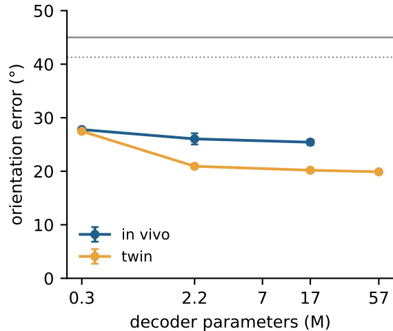
MICrONS orientation
