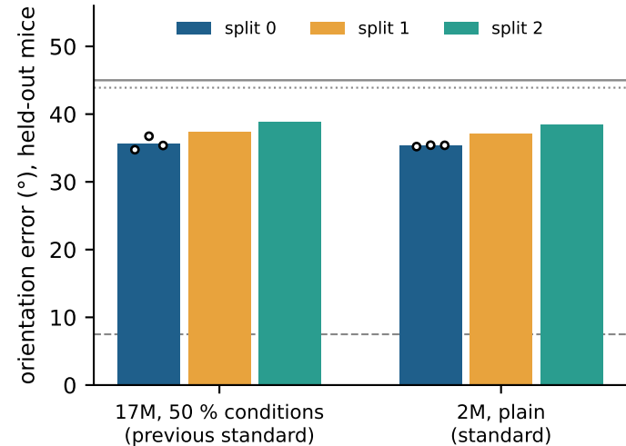
Allen orientation, `pooledcross`, by mouse split
