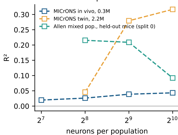
receptive field
