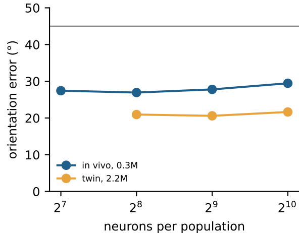
MICrONS orientation
