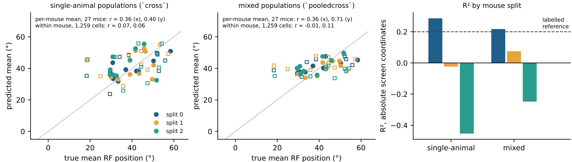
Fig. 4 Allen RF: what crosses animals is each animal's screen position, not the retinotopic layout within it
