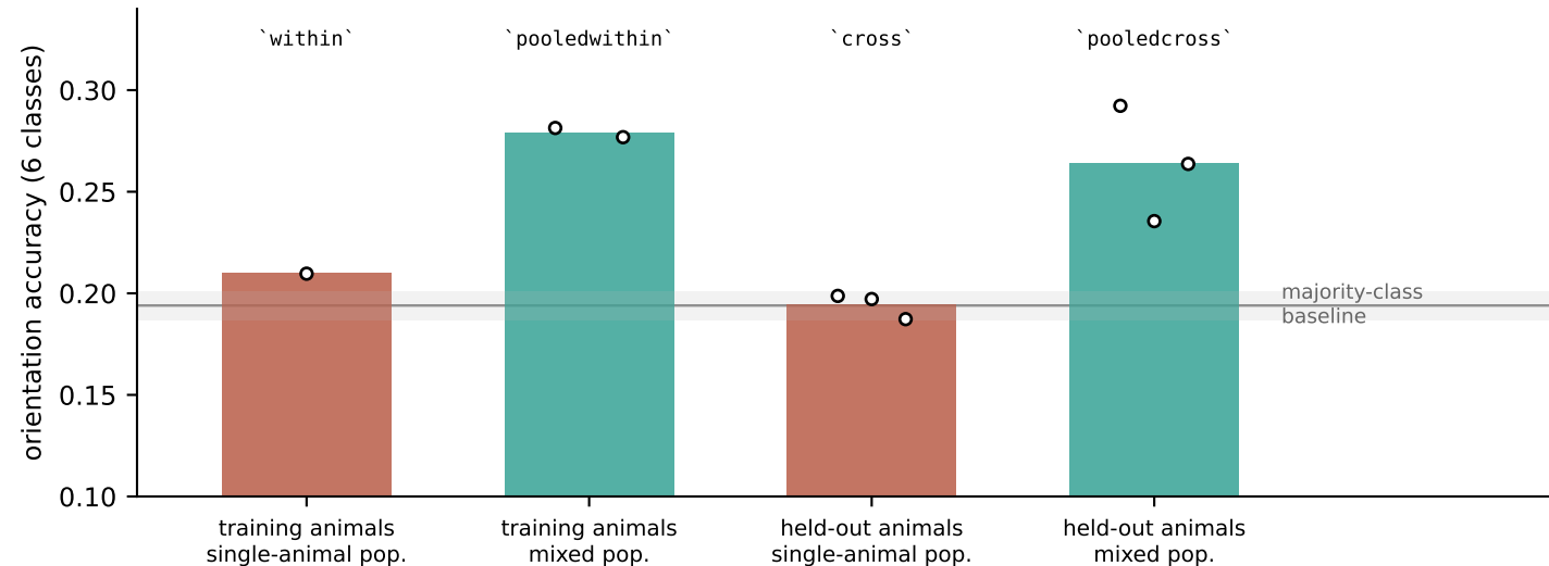
Fig. 5 Allen (33 mice, grating relations): orientation is readable only from populations that mix animals
