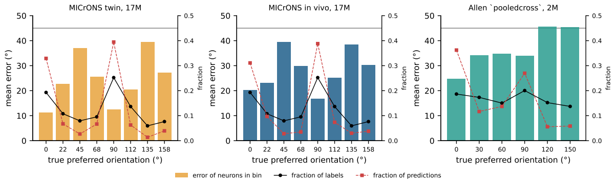
Figure A5: The readout is cardinal. Mean angular error of the neurons in each true-orientation bin (bars; grey line: 45° chance), with the fraction of labels (black) and of predictions (red) per bin, for the twin and in-vivo MICrONS decoders (neuron split 2) and the Allen pooledcross decoder. Cardinal orientations are decoded well, obliques near chance, and most predictions fall on 0° or 90°.
