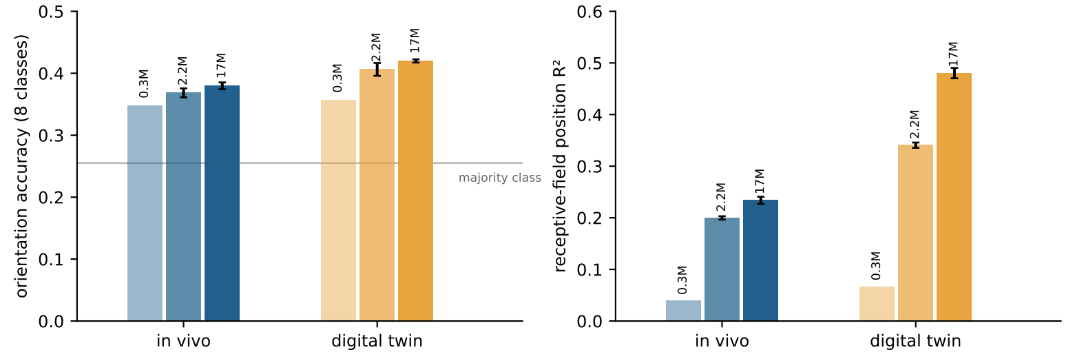
Fig. 1 MICrONS: per-neuron content decoded from the population correlation matrix alone (512 neurons, no labels, no reference)
