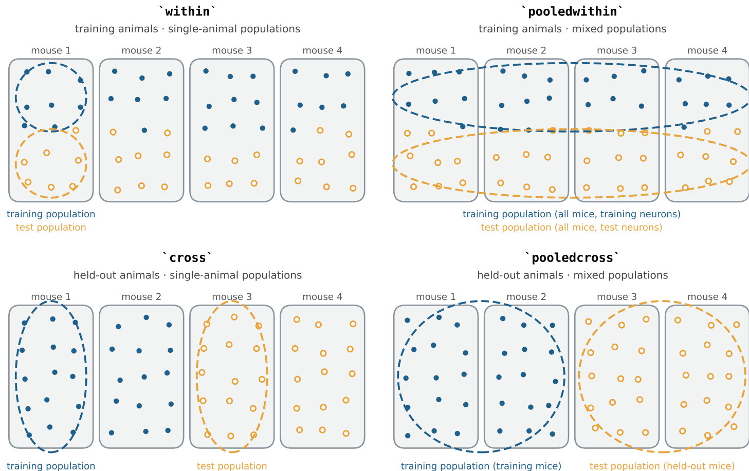
Fig. 3 Allen decoder regimes: where the test neurons come from \times what one population contains
