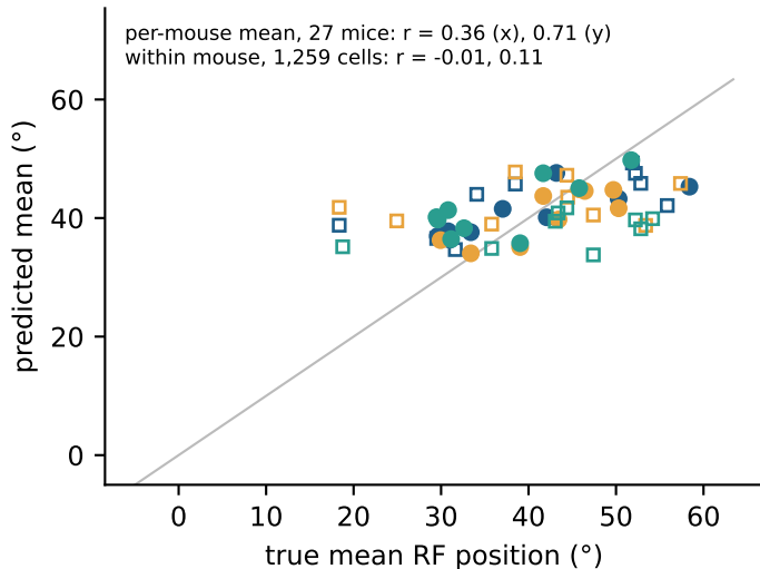
Fig. 5 Allen RF: what crosses animals is each animal's screen position, not the retinotopic layout within it single-animal populations (`cross`)
