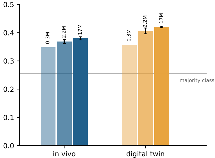
orientation accuracy (8 classes)
