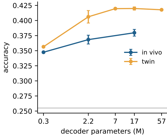
MICrONS orientation
