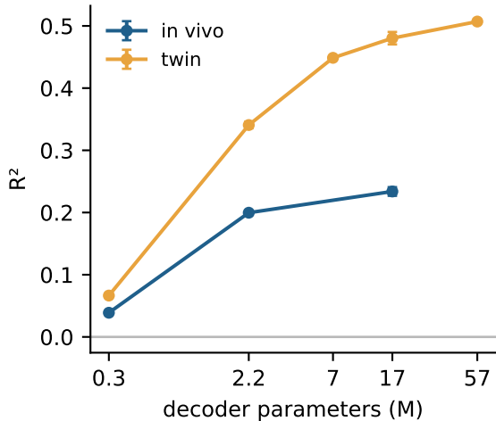
MICrONS RF (x, y)
