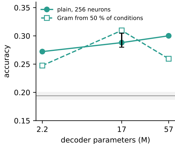
Allen orientation, held-out mice (split 0)
