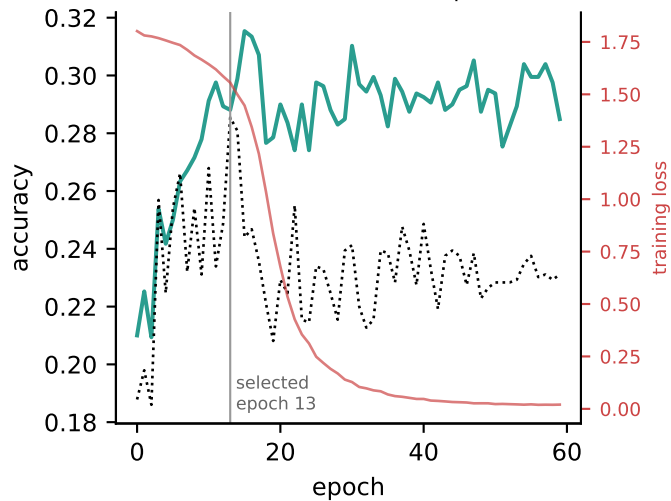
Allen orientation, 17M, plain
