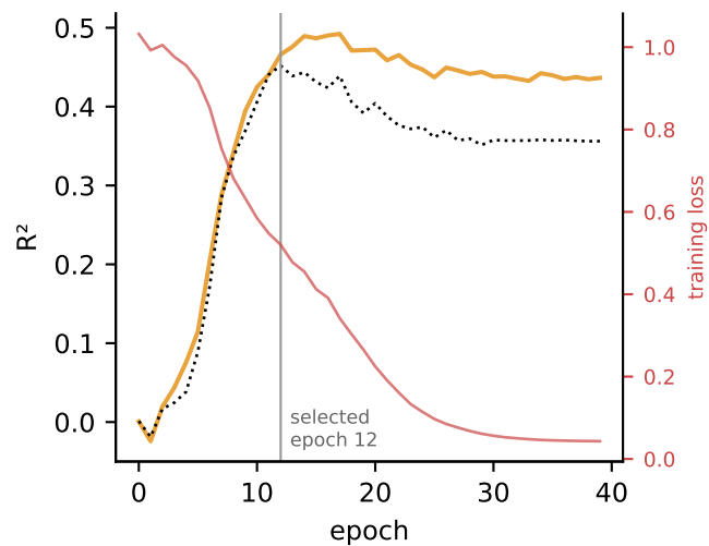
MICrONS twin RF, 17M
