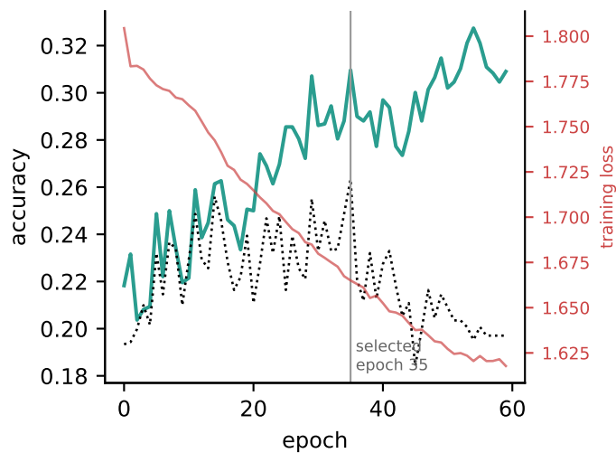
Allen orientation, 17M, 50 % conditions
