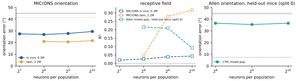
Figure A2: Population size. Test metric versus the number of neurons in each sampled population. Beyond 256 to 512 neurons the orientation error moves by at most 2°, up or down; twin receptive fields keep gaining slowly, Allen receptive fields lose.
