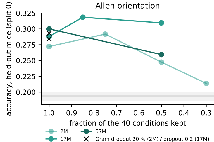
Fig. A3 Label-free relation augmentation: each training population's Gram from a random subset of stimulus conditions
