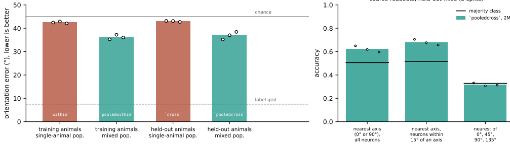
Figure 6: Allen, 33 mice, grating relations: orientation is readable only from populations that mix animals. Left: mean angular error; bars: mean over splits; points: the three splits; solid line: 45° chance; dashed line: the 7.5° label grid. Single-animal populations are 2° to 3° below chance whether the animal was seen in training or not; mixed populations are 7° to 10° below it in both rows. Right: coarse readouts of the mixed-population decoder on the held-out mice (three splits): correct cardinal axis for all cells and for the cells labelled 0° or 90°; the third bar, nearest of 0°, 45°, 90°, 135° and is shown for comparison with MICrONS; black ticks: majority class.
