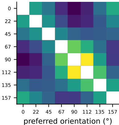
in-vivo class-Gram (8 × 8)
