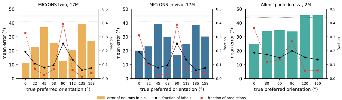
Figure 3: The readout is cardinal. Mean angular error of the neurons in each true-orientation bin (bars; grey line: 45^\circ chance; dotted: best constant), with the fraction of labels (black) and of predictions (red) per bin, for the twin and in-vivo MICrONS decoders (neuron split 2) and the Allen pooledcross decoder. Cardinal orientations are decoded well, obliques near chance, and most predictions fall on 0^\circ or 90^\circ .
