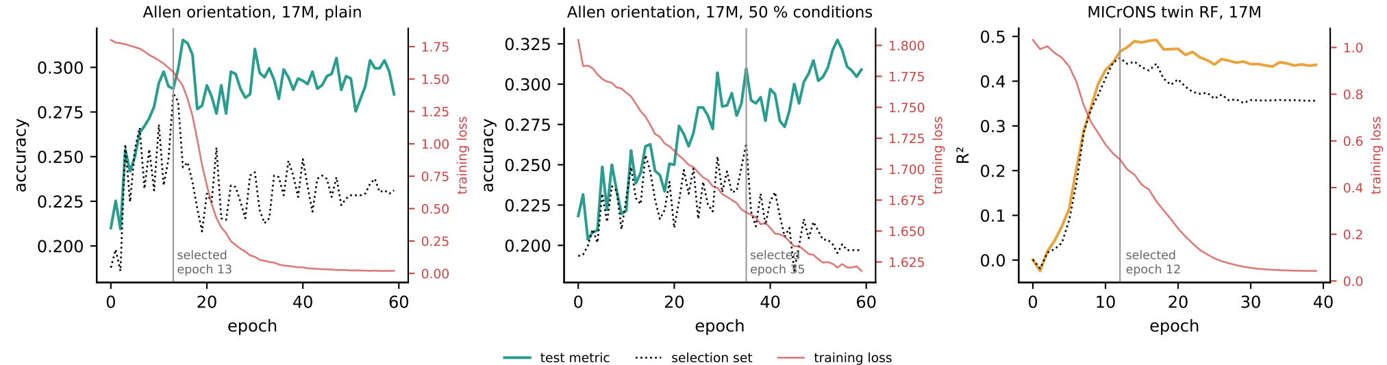
Fig. A4 Every large run memorises its training neurons; the reported score is the epoch chosen on a held-out selection set
