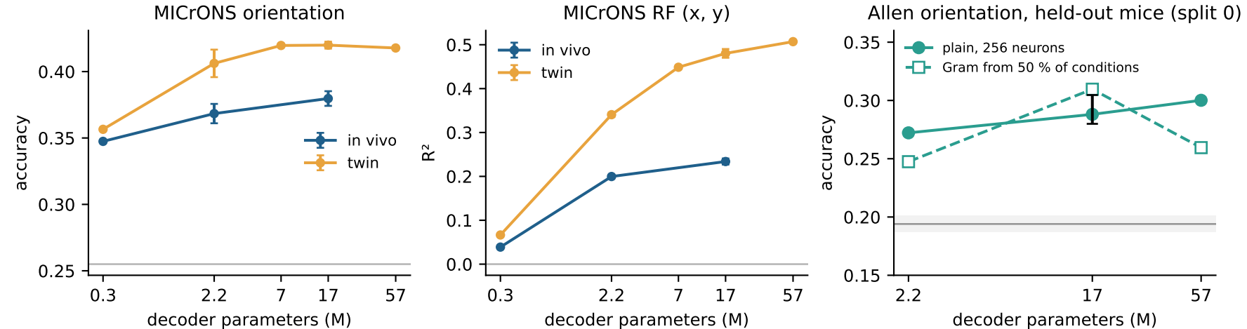
Fig. A1 Capacity: RF keeps gaining with model size, orientation does not (label counts 11,326 vs 5,287 in MICrONS; 5,529 in Allen)
