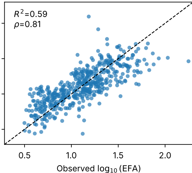
Combined
