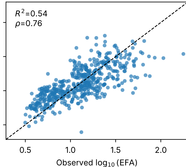
Chemistry only
