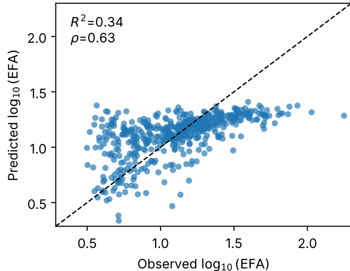
DFT only
