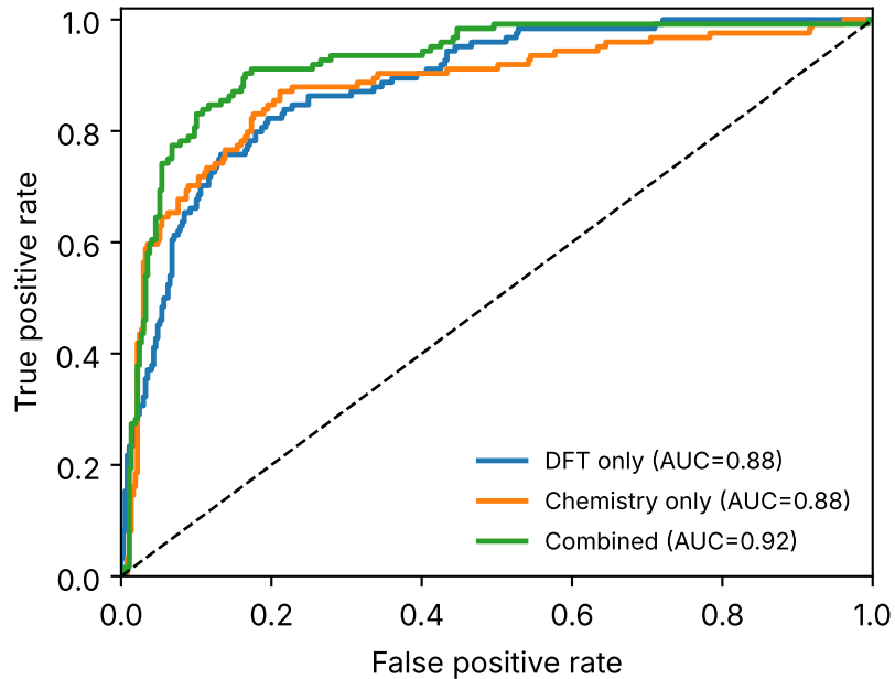
ROC curve
