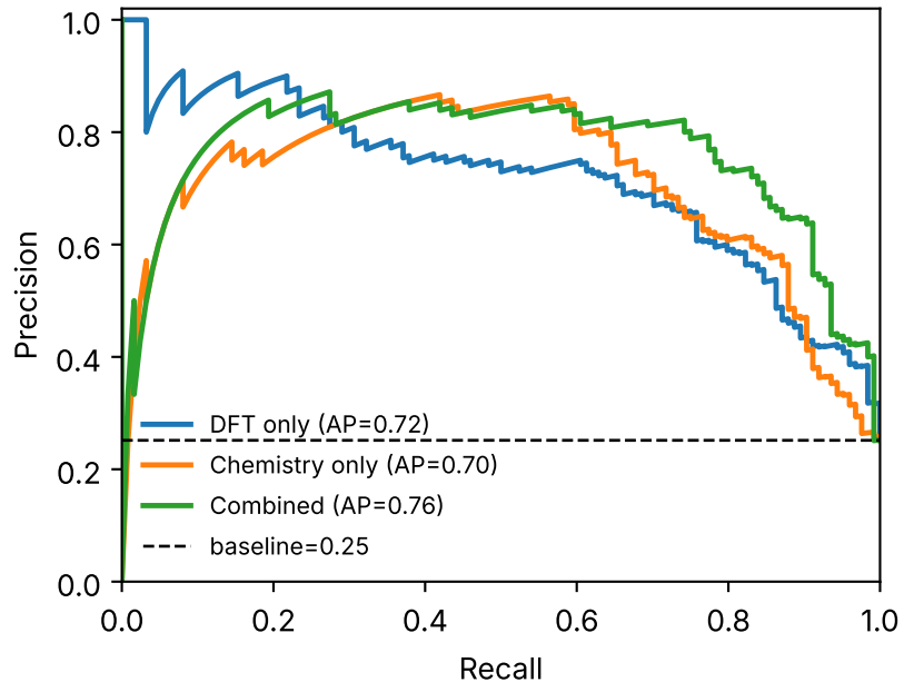
Precision-recall curve
