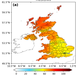
Dec 2017 — Nov 2018 Mean PM_{2.5} ( \mu\text{g}/\text{m}^3 ) MUSICAv0
