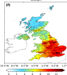
Dec 2017 — Nov 2018 Mean PM_{2.5} ( \mu\text{g}/\text{m}^3 ) UKAQR
