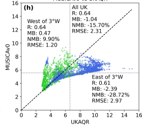
Dec 2017 — Nov 2018 Mean PM_{2.5} ( \mu\text{g}/\text{m}^3 ) MUSICAv0 vs UKAQR
