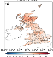
Dec 2017 — Nov 2018 Mean PM_{2.5} ( \mu\text{g}/\text{m}^3 ) MUSICAv0 - UKAQR
