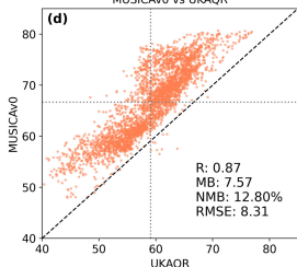
Dec 2017 — Nov 2018 Mean PM_{2.5} ( \mu\text{g}/\text{m}^3 ) MUSICAv0 vs UKAQR
