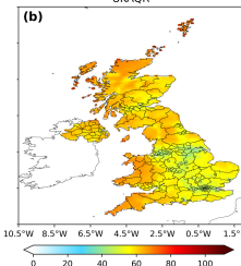
Dec 2017 — Nov 2018 Mean PM_{2.5} ( \mu\text{g}/\text{m}^3 ) UKAQR
