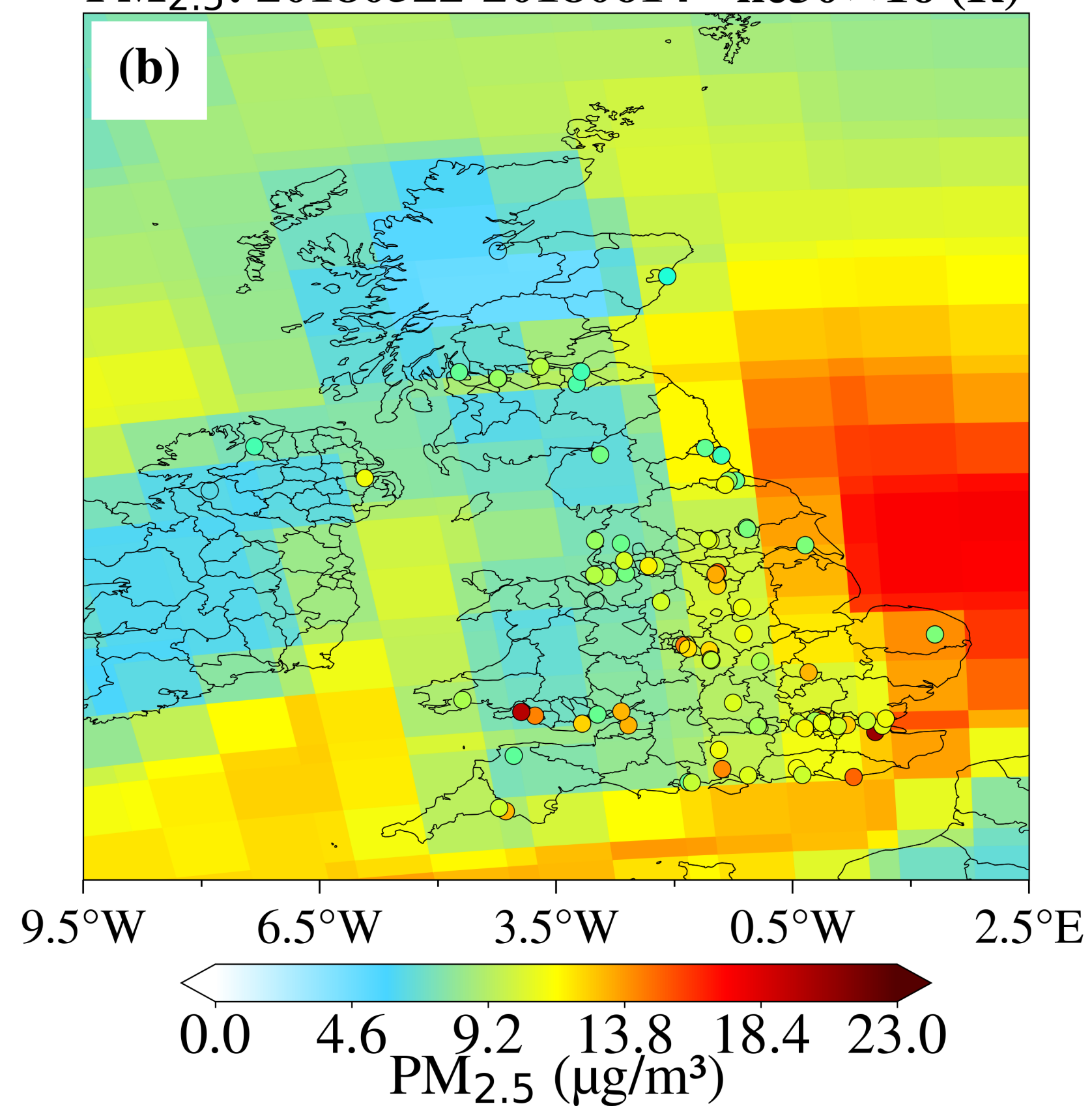
PM 2.5 : 20180522-20180614 ne30×16 (R)
