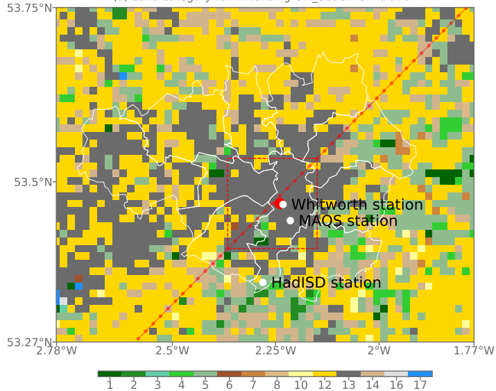
(a) Land category for initializing GM_SLUCM simulation
