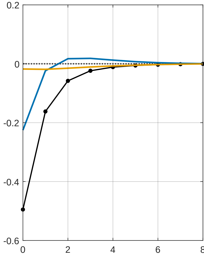
Counterfactual
