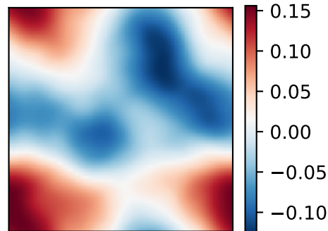
F-SPDENO t=0.25
