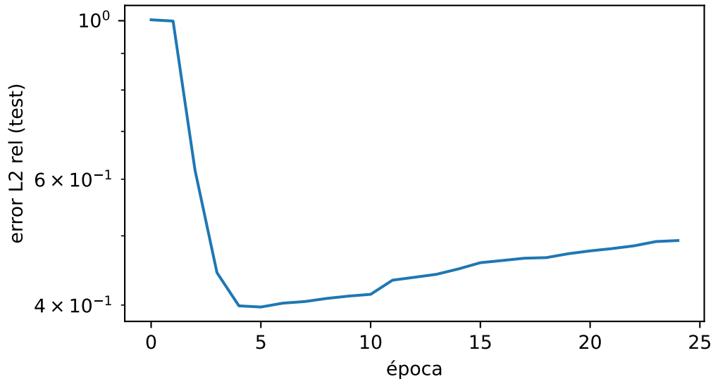
Entrenamiento F-SPDENO 2D ((X0,W)->X)
