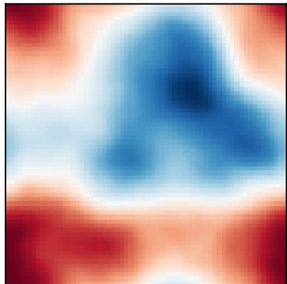
(X0,W)->X t=0.00
