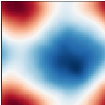
(X0,W)->X t=0.12
