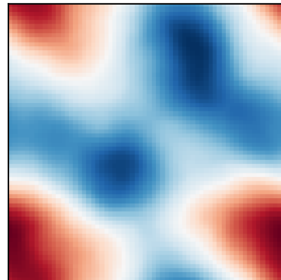
(X0,W)->X t=0.37
