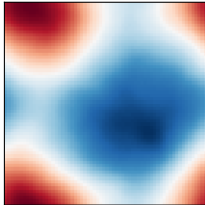
(X0,W)->X t=0.25
