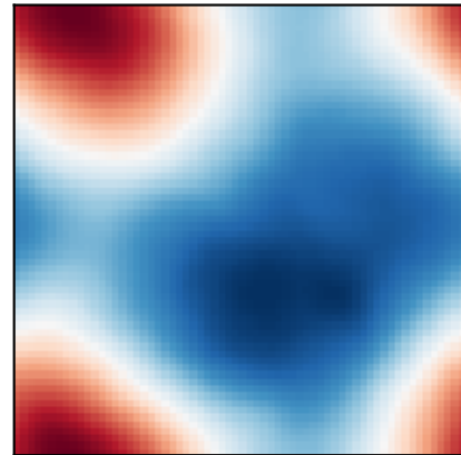
(X0,W)->X t=0.50
