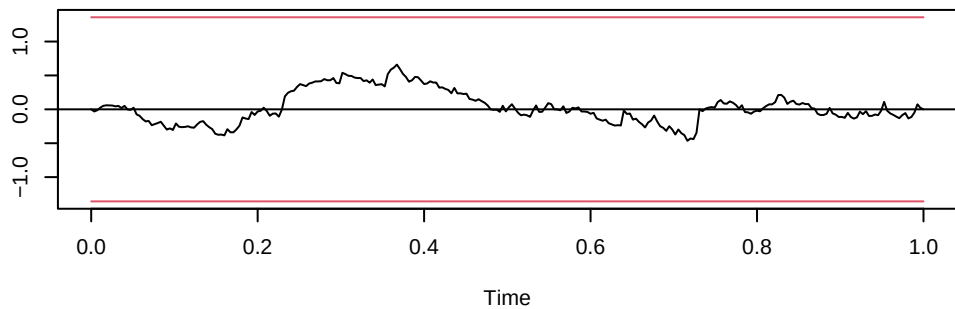
OLS-CUSUM of equation vix
