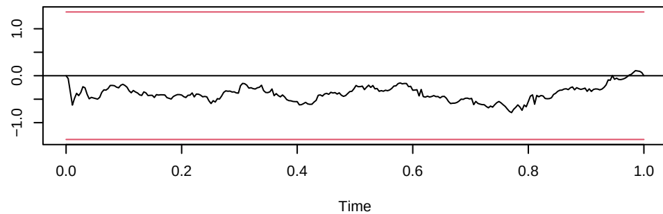
OLS-CUSUM of equation selic
