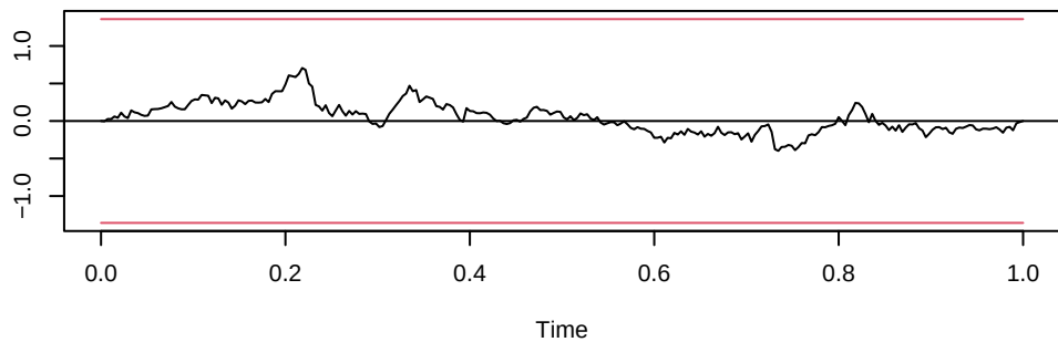
OLS-CUSUM of equation comm
