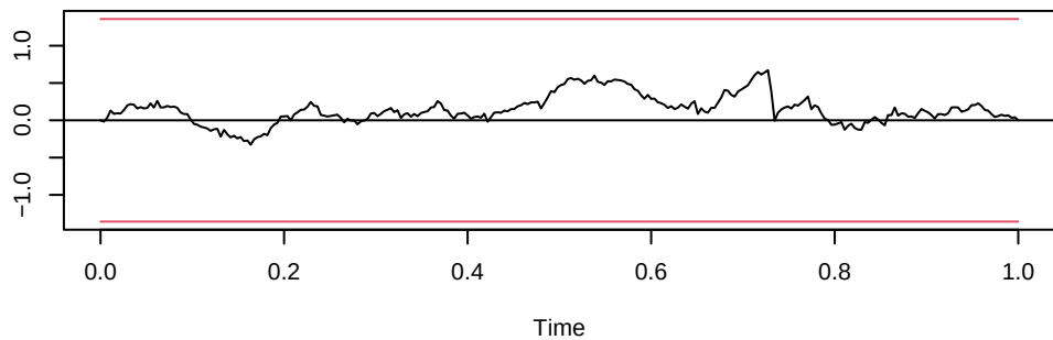
OLS-CUSUM of equation hiato
