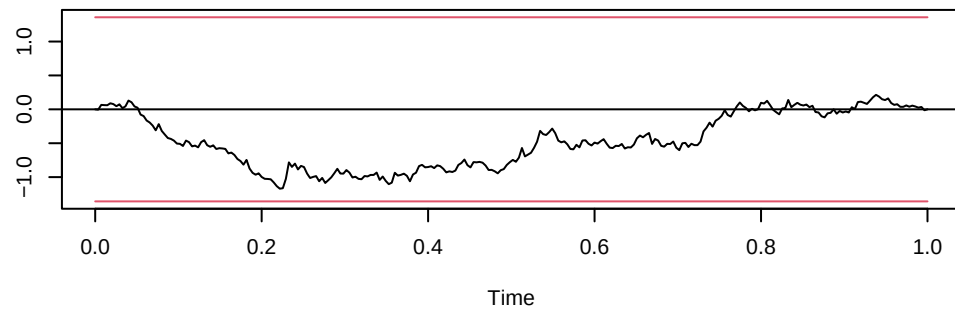
OLS-CUSUM of equation cambio
