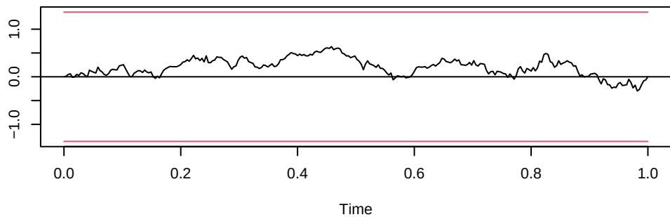
OLS-CUSUM of equation pimp
