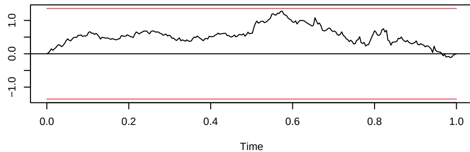
OLS-CUSUM of equation ipca
