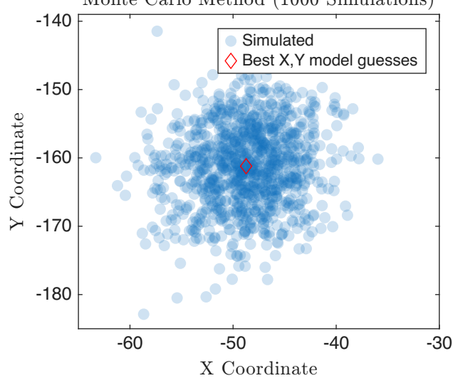
Monte Carlo Method (1000 Simulations)
