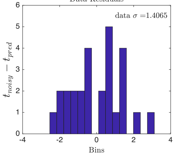
Data Residuals
