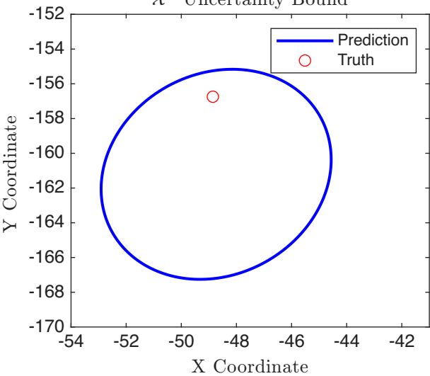
\chi^2 Uncertainty Bound
