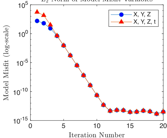
L_2 Norm of Model Misfit Variables
