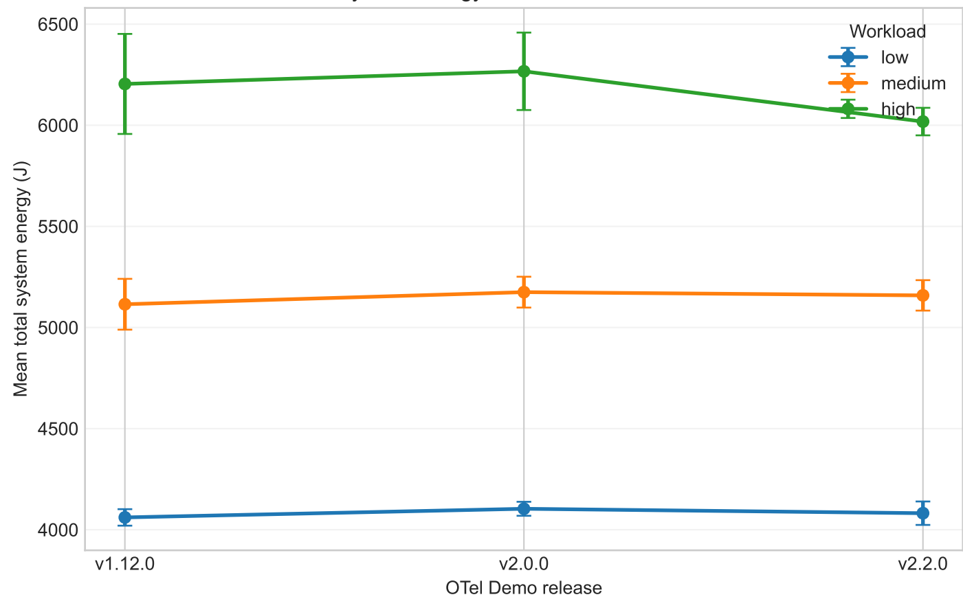
Total system energy across OTel Demo releases
