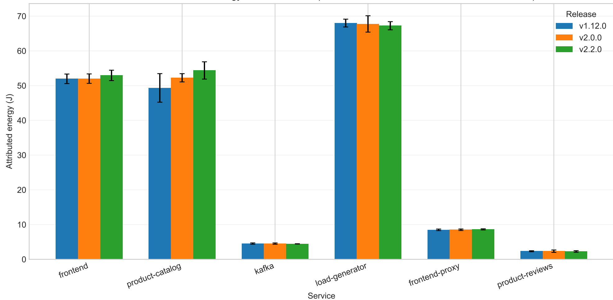
Service-level attributed energy across releases (absolute, mean \pm std, workstation, medium, M1)
