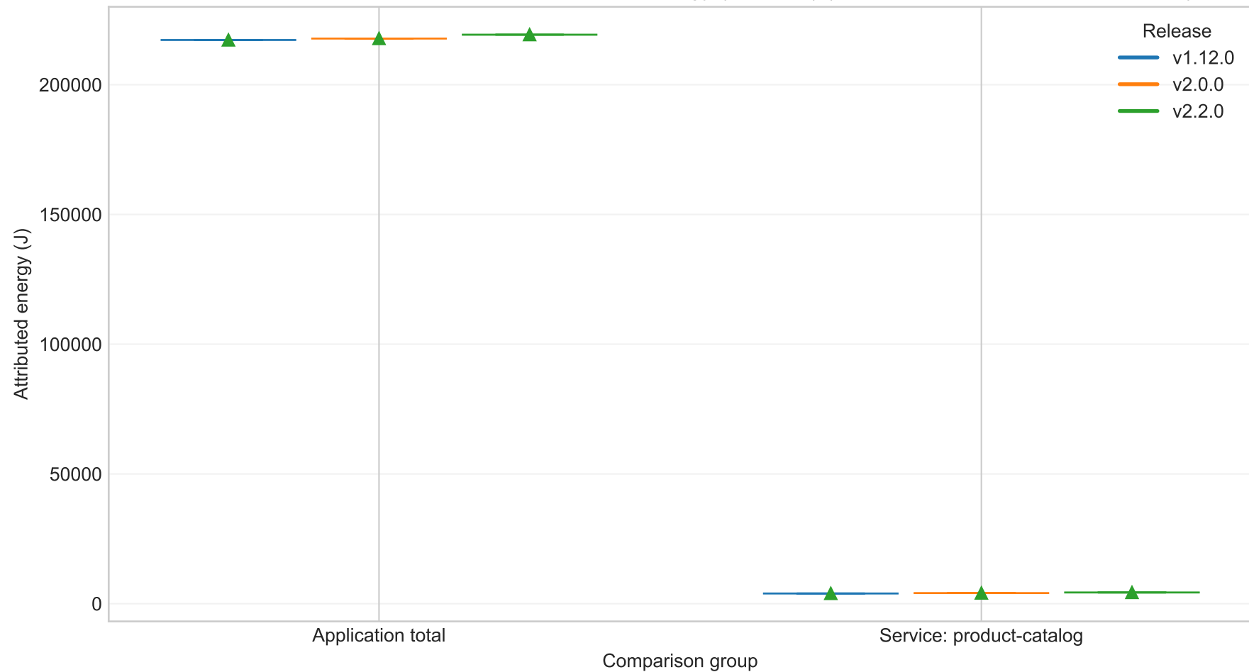
Application total vs selected services attributed energy (boxplots) (ec2, workload=medium, model=M2)
