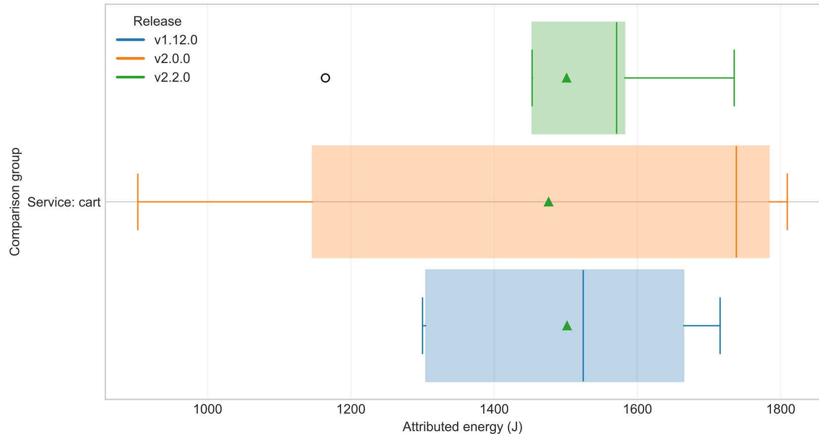
Selected service attributed energy (iteration-level boxplots, rotated) (ec2, service=cart, workload=medium, model=M1)
