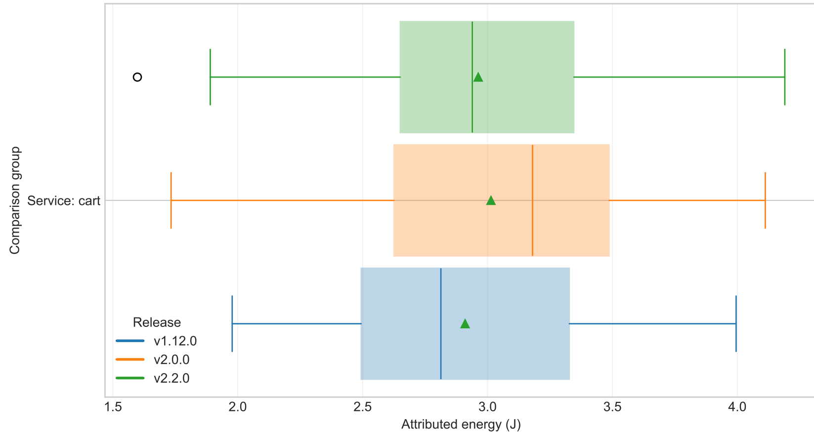
Selected service attributed energy (iteration-level boxplots, rotated) (workstation, service=cart, workload=medium, model=M1)
