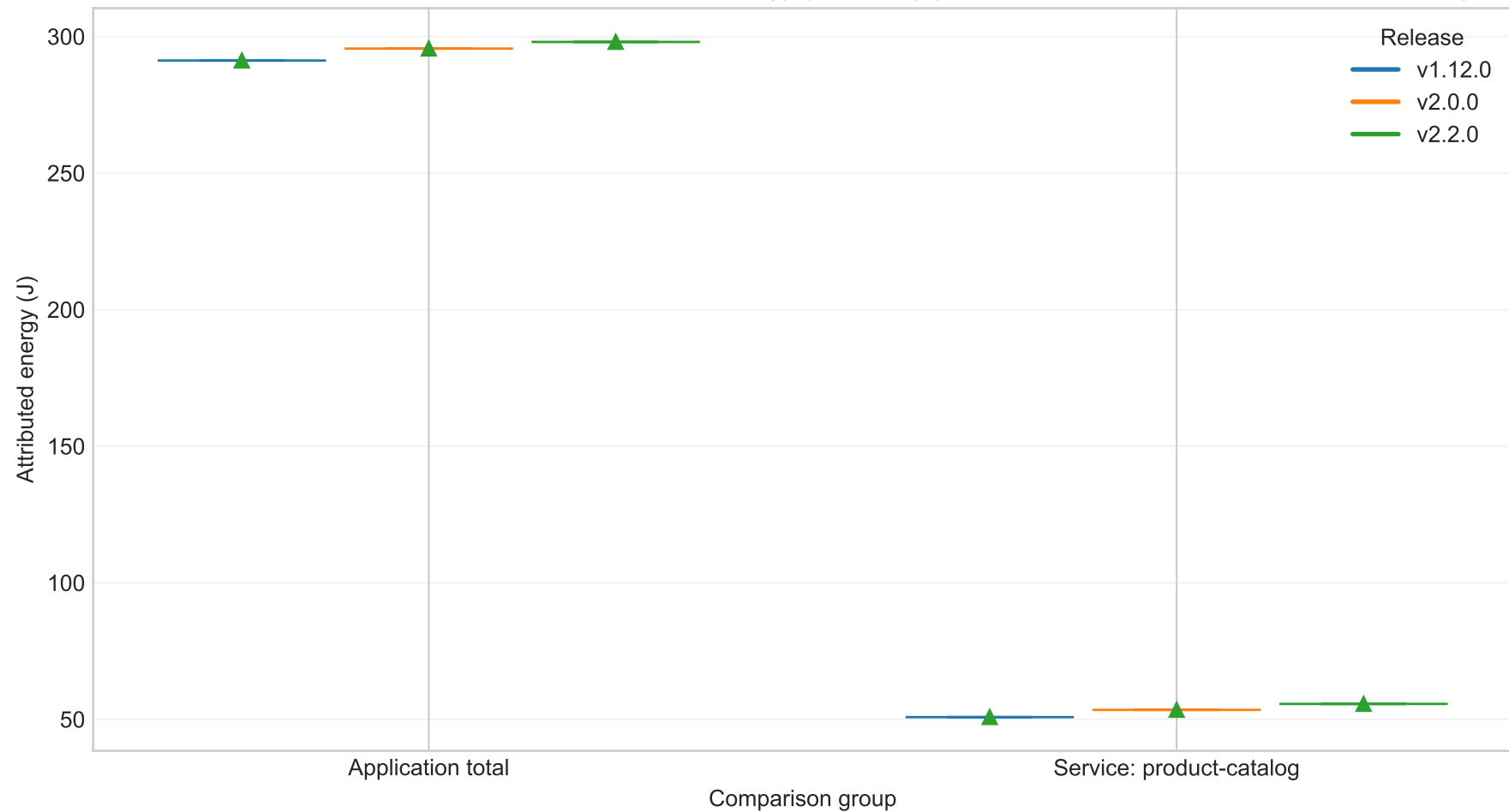
Application total vs selected services attributed energy (boxplots) (workstation, workload=medium, model=M2)
