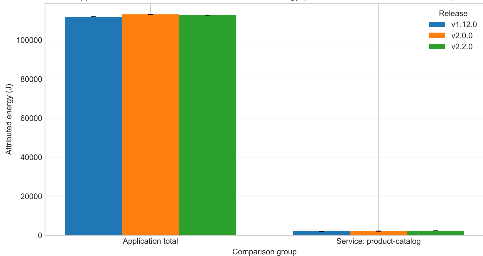
Application total vs selected services attributed energy (ec2, workload=medium, model=M1)
