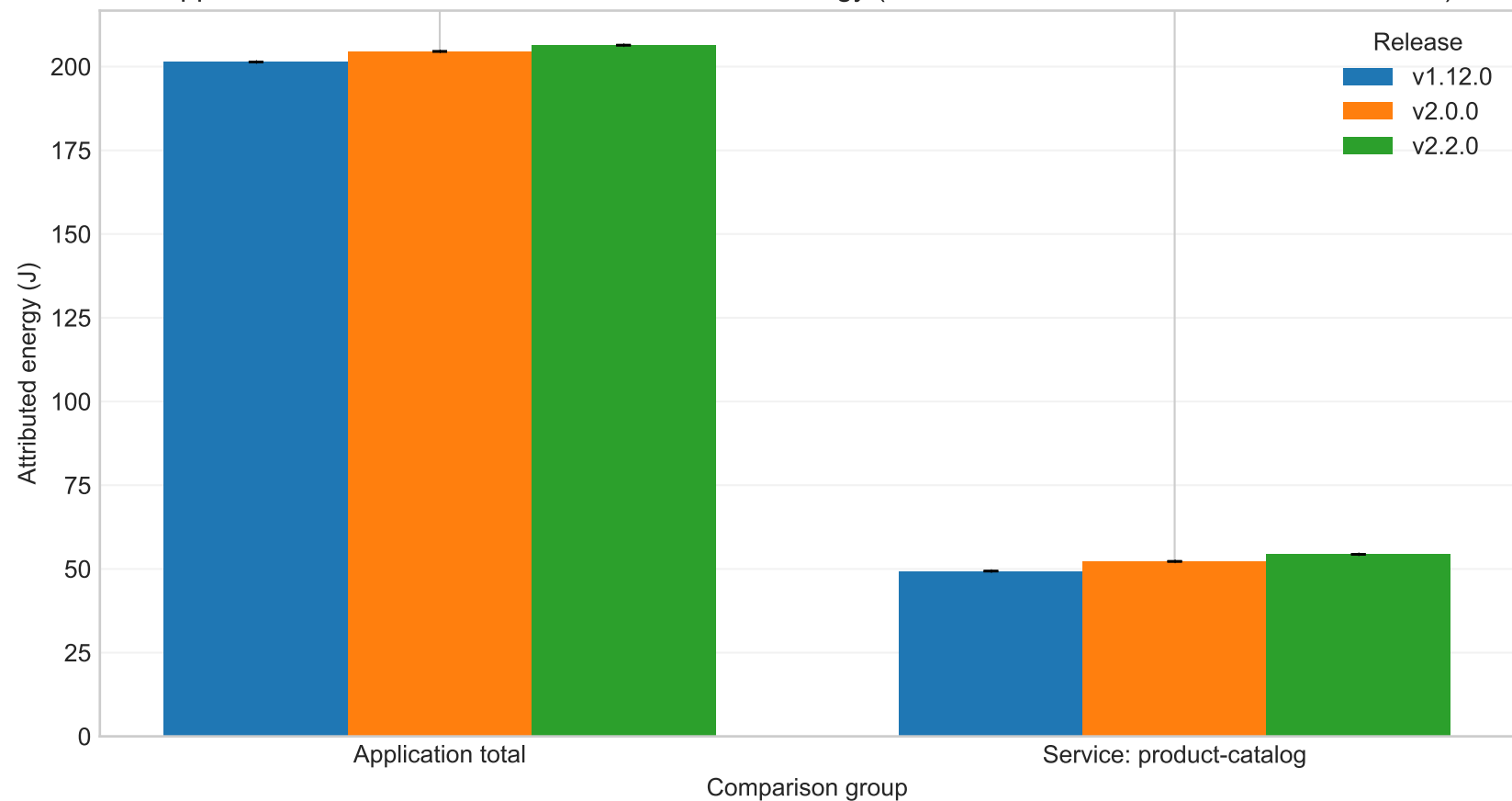
Application total vs selected services attributed energy (workstation, workload=medium, model=M1)
