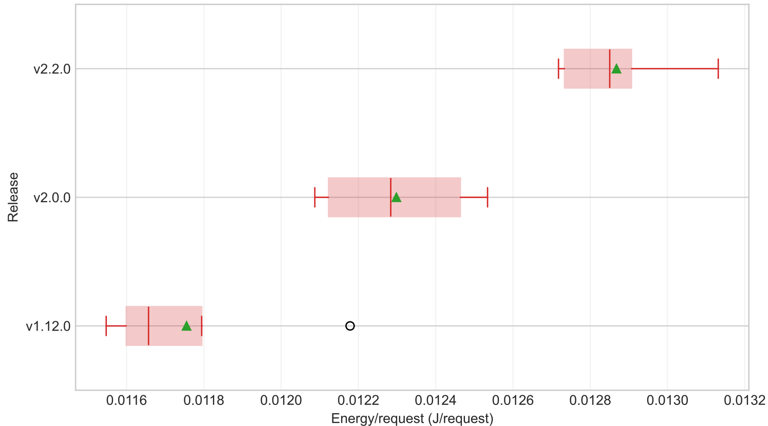
Fixed-util selected service EPR by release (ec2, service=product-catalog, workload=medium, model=M2)
