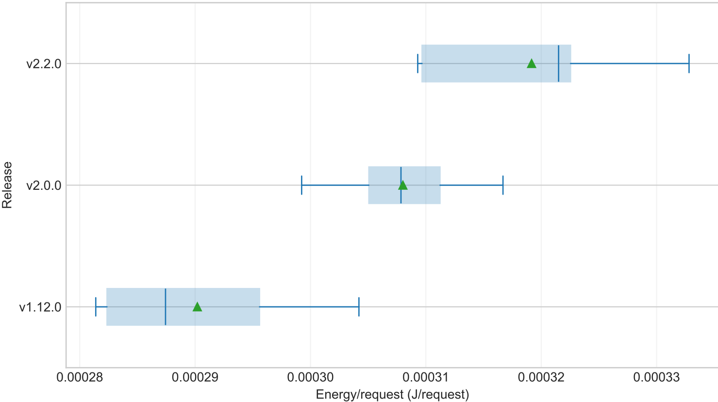
Fixed-util selected service EPR by release (workstation, service=product-catalog, workload=medium, model=M1)
