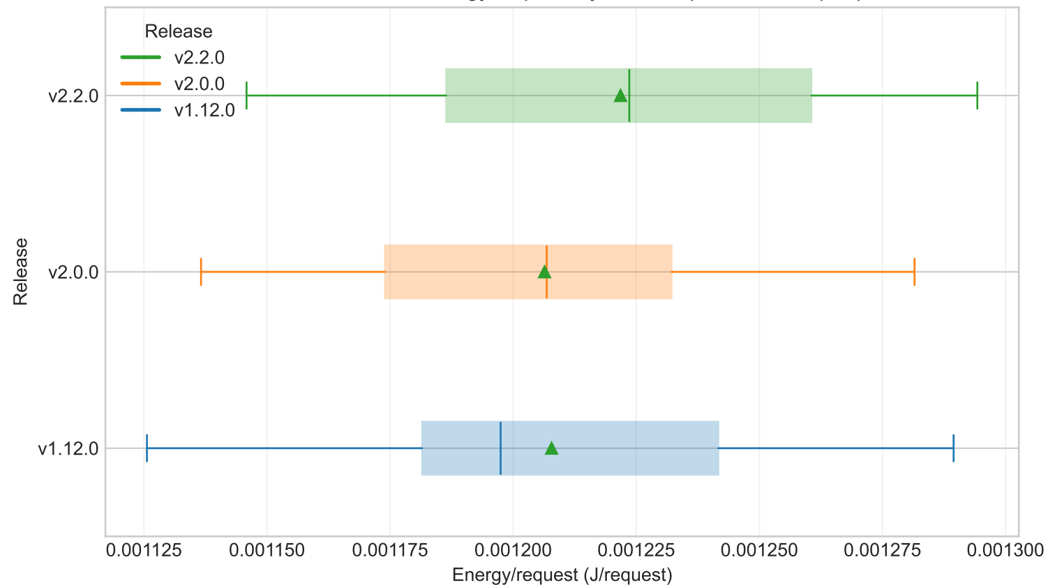
Fixed-utilisation energy/request by release (workstation, p80)
