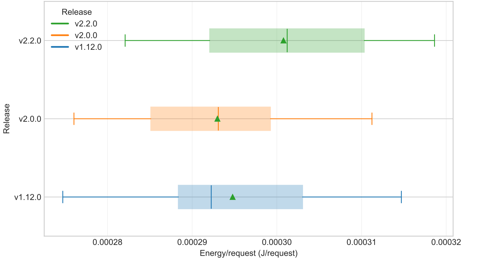
Fixed-util selected service EPR by release (workstation, service=product-catalog, workload=medium, model=M1)
