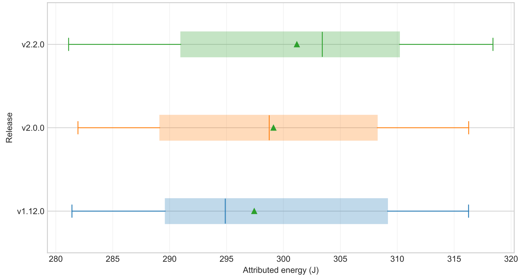
Total application energy by release (workstation, workload=medium, model=M2)
