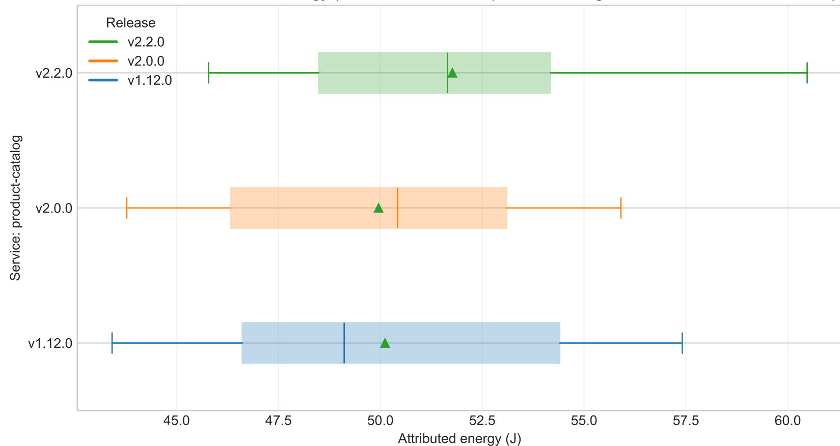
Selected service attributed energy (workstation, service=product-catalog, workload=medium, model=M1)
