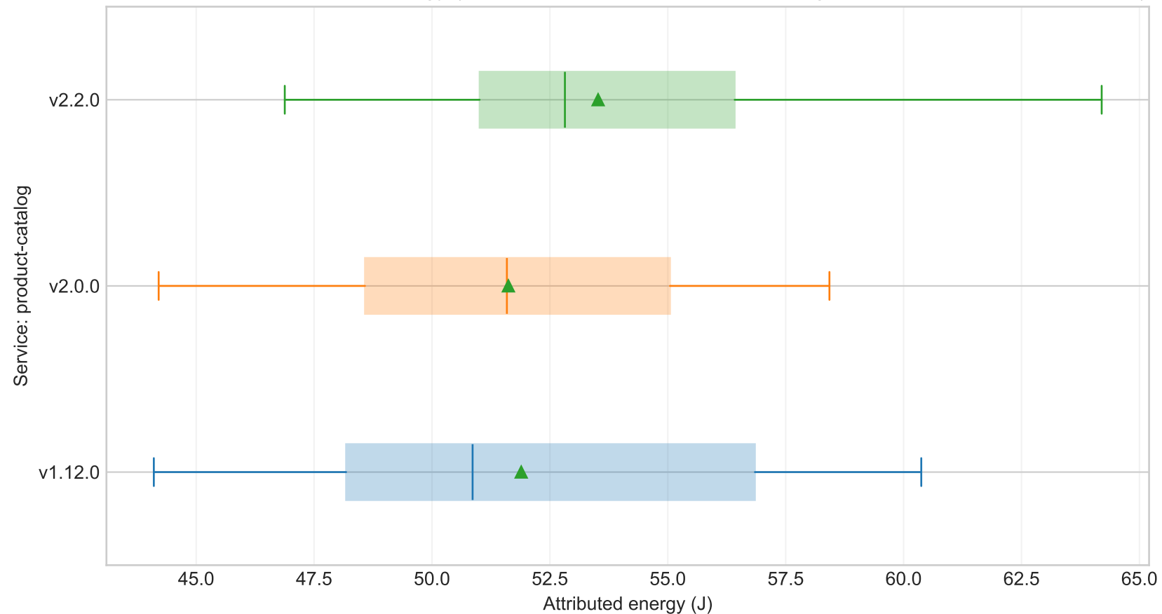
Selected service attributed energy (workstation, service=product-catalog, workload=medium, model=M2)
