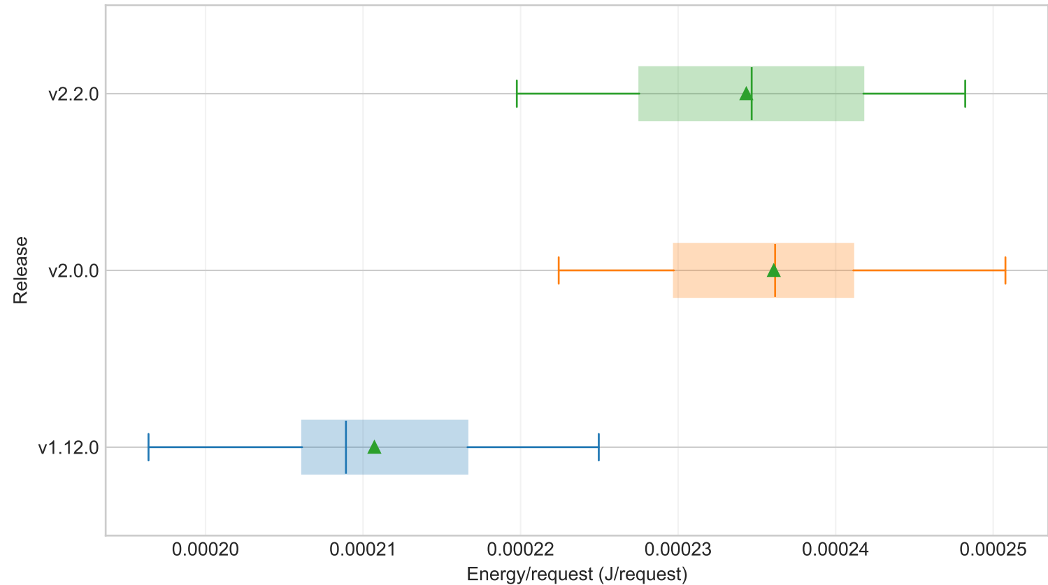
Fixed-util selected service EPR by release (workstation, service=product-catalog, workload=medium, model=M2)
